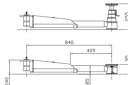
Short arm
