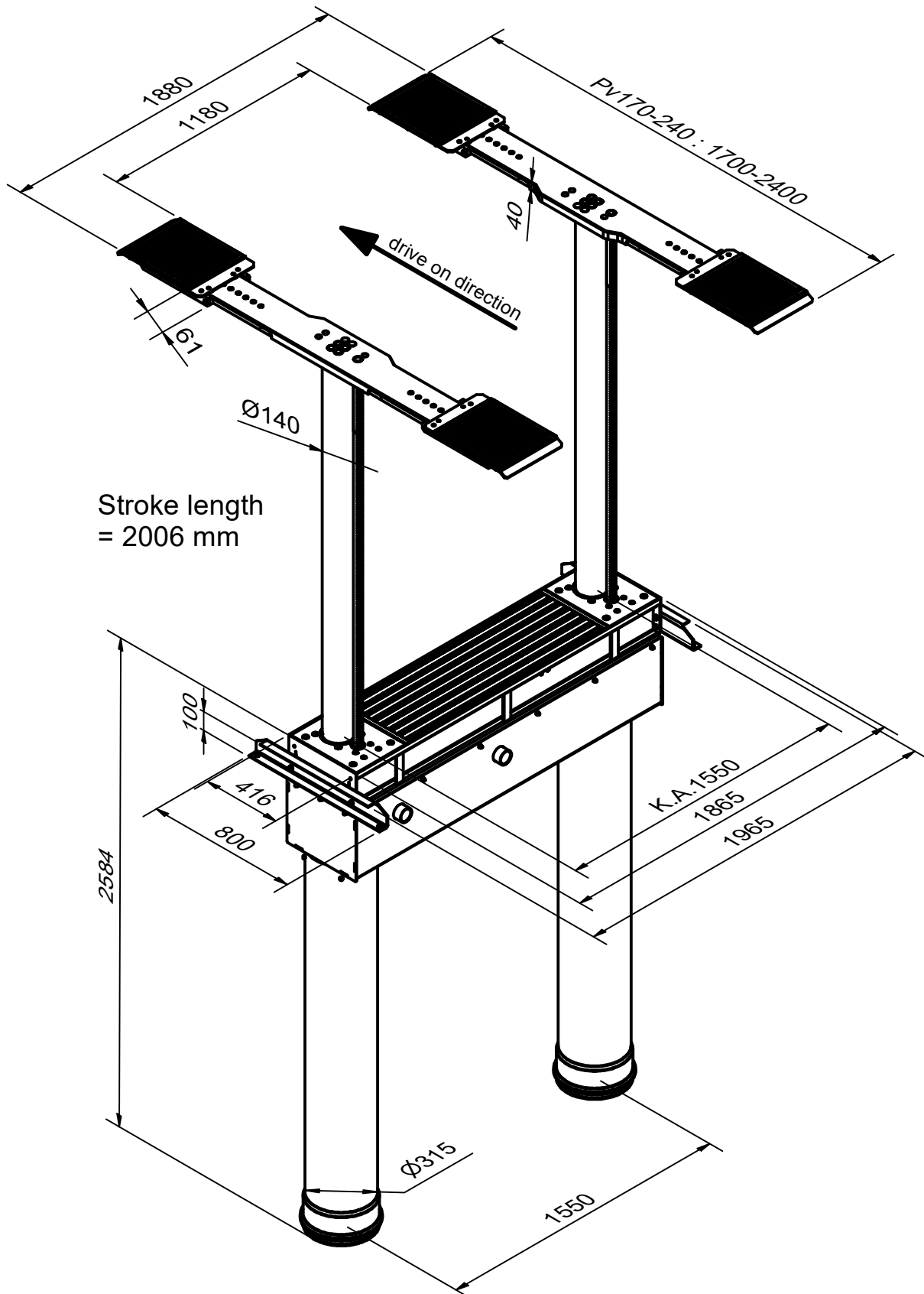
Dimensional sketch including drive-over heights
